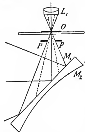
FIG. 40.—Mirror Illumination.
