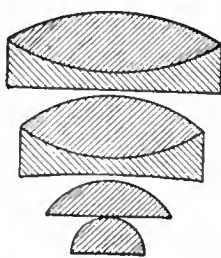
FIG. 35.—Achromatic objective for homogeneous immersion.
