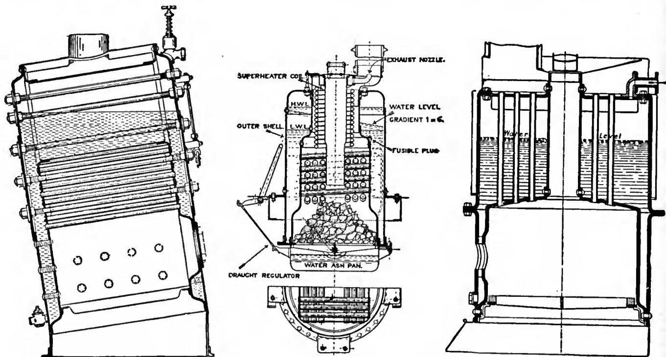
FIGS. 16, 17, 18.—Fig. 16 shows the Toward Vertical Boiler, fig. 17 Alley & MacLellan's Sentinel Water-tube Boiler, and fig. 18 the Vertical Smoke-tube Boiler fitted on Leyland Steam Wagons. The smoke tubes in the last-named boiler are provided with copper sleeves to prevent corrosion.
