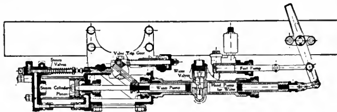
FIG. 22.—The Sheppee Combined Steam-driven or Hand-operated Water-pump.
