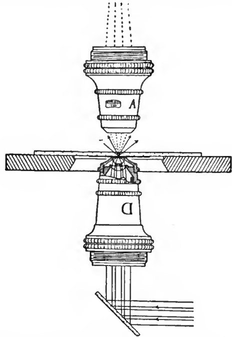
FIG. 45.—Path of Rays for dark-ground illumination with fixed diaphragm in the objective.
