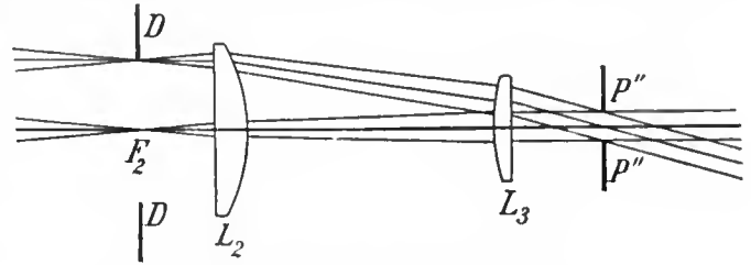
FIG. 37.—Ramsden Eyepiece.
