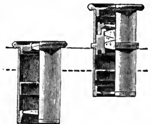
FIG. 39.—Compensating Eyepieces (Zeiss).
