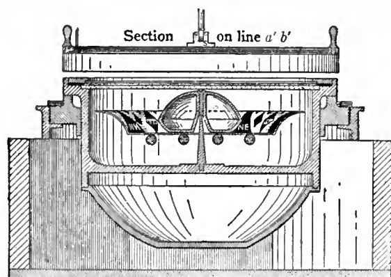
FIG. 5.—Abbe's Marine Nephoscope. Vertical Section.
