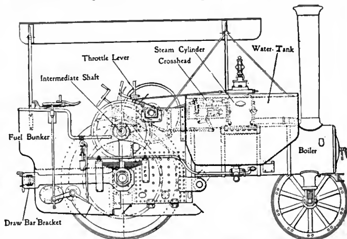
FIG. 25.—Foster's "Wellington" Compound Steam Tractor with outside spring suspension.
