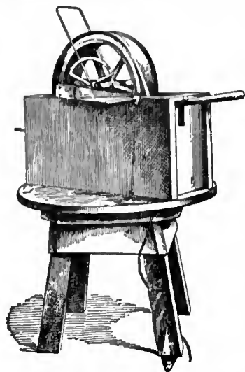
FIG. 7.—Marvin Kite Reel for hand power.
