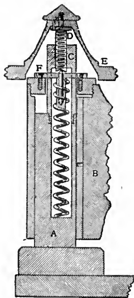
FIG. 51.—Micrometer Screw Adjustment of Leitz.
