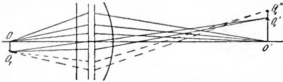
FIG. 29.—The lens is spherically corrected for OO' , but the sine-condition is not fulfilled. Hence the different magnifications of a point O_1 beyond the axis.
