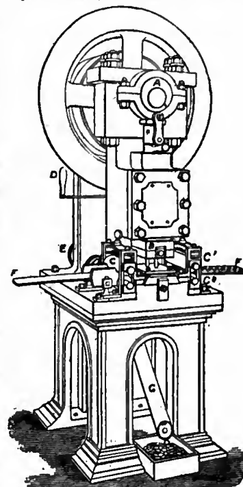
FIG. 3.—Cutting Machine.
