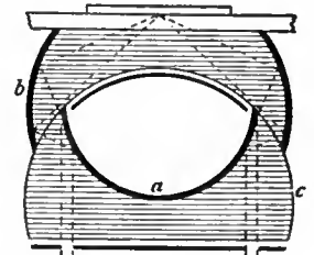
FIG. 47.—Siedentopf's Cardioid Condenser.
