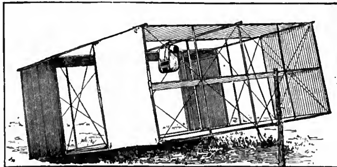
FIG. 6.—Marvin-Hargrave Kite, with Meteorograph in position.
