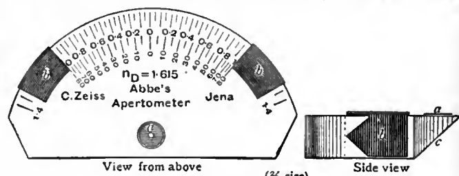
FIG. 56.—Abbe's Apertometer (Zeiss).
