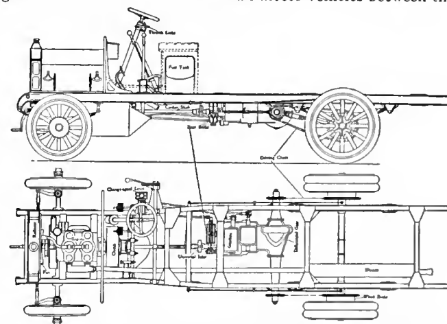
FIG. 28.—Halley's Van or Lorry Chassis with 20 h.p. Engine.
