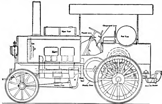
FIG. 37.—45 h.p. Thornycroft Military Oil Tractor.
