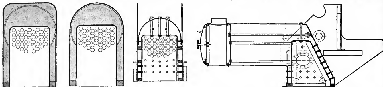
FIGS. 12-15.—Fig. 12 shows the Belpaire type of fire-box construction as compared with the more usual type shown in fig. 13. Fig. 14 and fig. 15 show the form of locomotive boiler fitted by Sidney Straker & Squire, Ltd. The back of the fire-box is sloped so as to accommodate the gear shafts without unduly lengthening the frame.
