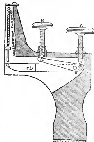
FIG. 53.—Double Lever Adjustment of Watson & Sons.
