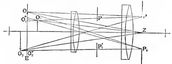
FIG. 15.—Entocentric transmission through a microscope objective.
