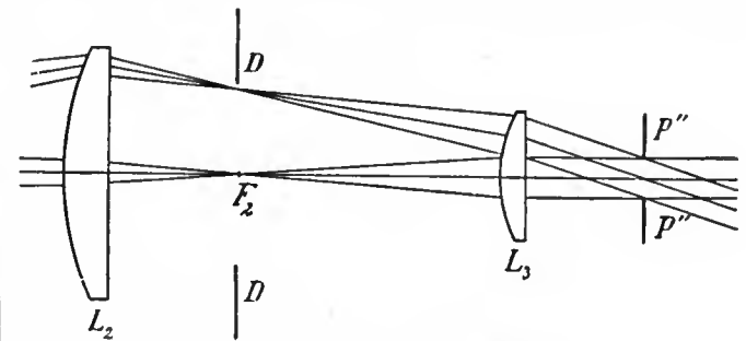
FIG. 38.—Huygenian Eyepiece.
