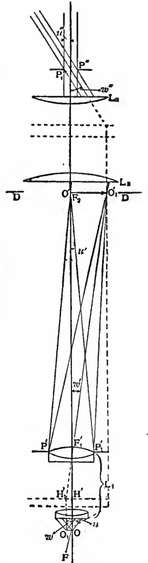
FIG. 13.—Ray transmission in compound microscope with a positive ocular.
