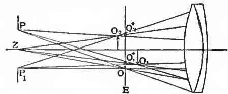
FIG. 16.—Hypercentric transmission in a microscope objective.
