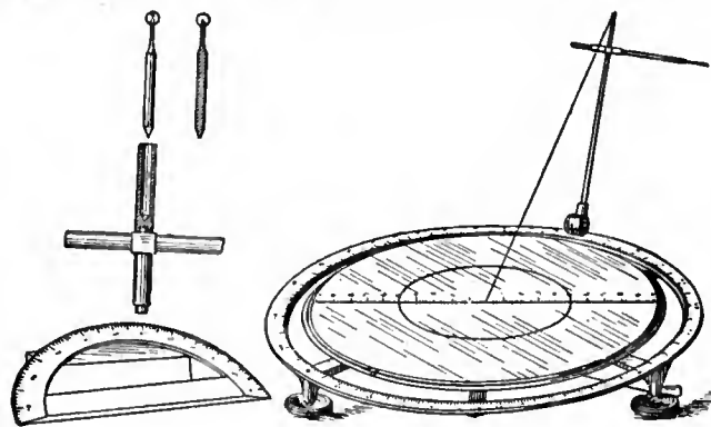
FIG. 2.—Marvin's Nephoscope.
