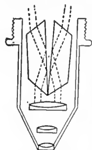
FIG. 48.—Riddell's Prisms.
