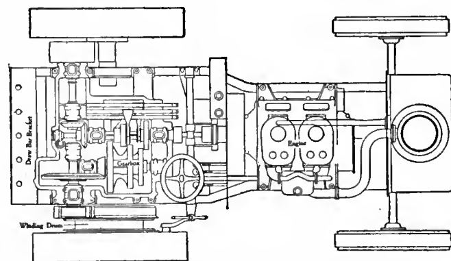
FIG. 36.—Marshall's 30 h.p. Agricultural Tractor.
