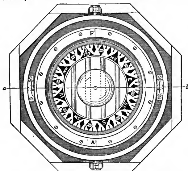
FIG. 4.—Abbe's Marine Nephoscope. Horizontal Projection of Compass.
