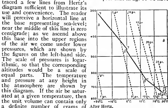
FIG. 10.—Diagram for Graphic Method of following Adiabatic Changes.
