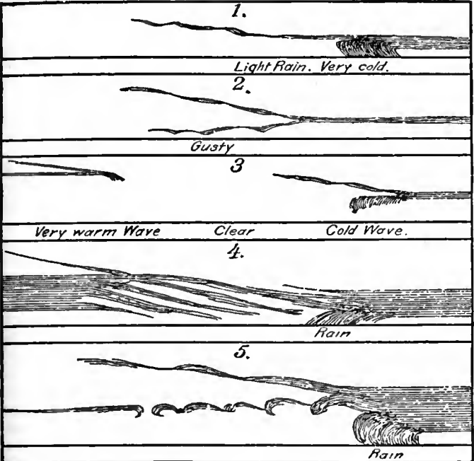
After Brillouin. FIG. 11.—Diagram illustrating Clouds due to Mixture.
