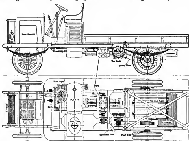
FIG. 24.—The Sheppee "Steam-gas" or Superheated Steam Vehicle.
