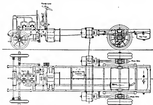
FIG. 32.—The Hallford-Stevens Petrol-electric Chassis.
